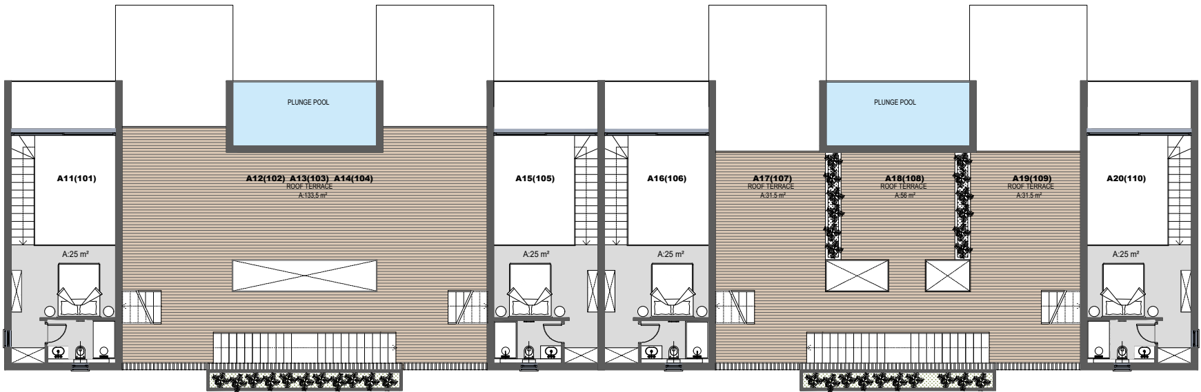
MEZZANINE PLAN
